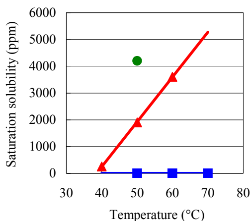
Fig. 3 Saturation solubility against T behenic acid(●) ;erucamide (▲) ;behenamide (■)
