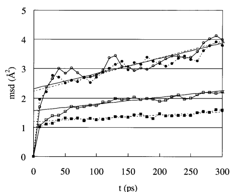
Fig. 5 Mean square displacement of UV-stabilizers as a function of time; Tinuvin 329: (□, ■); Tinuvin P: (○, ●). The straight lines show the least-squares fit by using data from 60 to 200ps.
