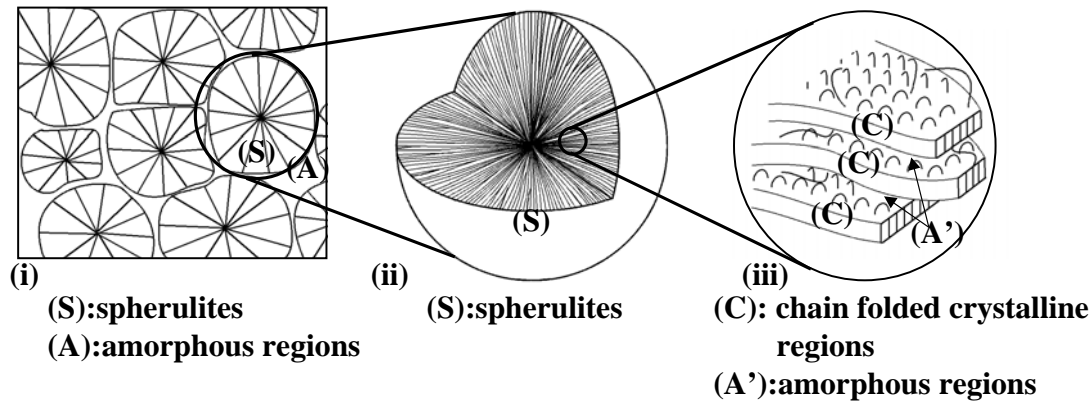
Fig. 1 Internal structure of isotactic polypropylene: (i) spherulites (S) and amorphous regions (A) among spherulites in iPP film (ii) internal structure of a spherulite(S) (iii) the chain folded crystalline regions (C) and amorphous regions (A') among the chain folded crystalline regions.
