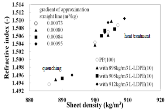
FIG. 13. Relationship between sheet density and refractive index for various metallocene L-LDPE blended PP sheets .
