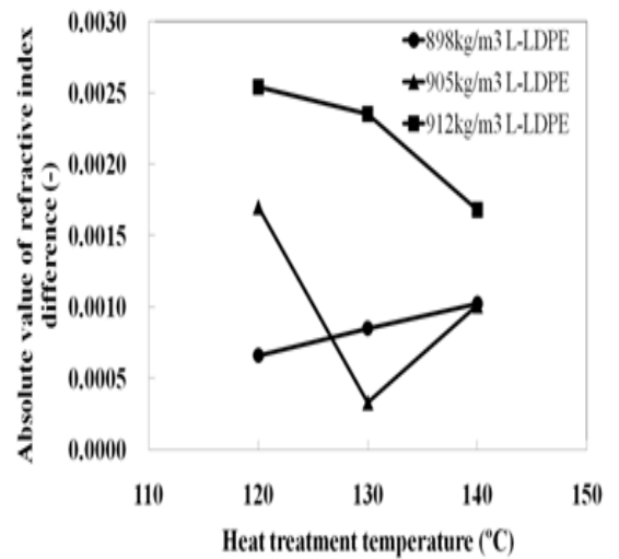
FIG. 16. Relationship between absolute value of refractive index difference of PP sheet and L-LDPE blended sheet and heat treatment temperatures for various metallocene L-LDPE blended PP sheets.
