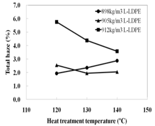
FIG. 15. Relationship between transparency and heat treatment temperatures for various metallocene L-LDPE blended PP sheets.
